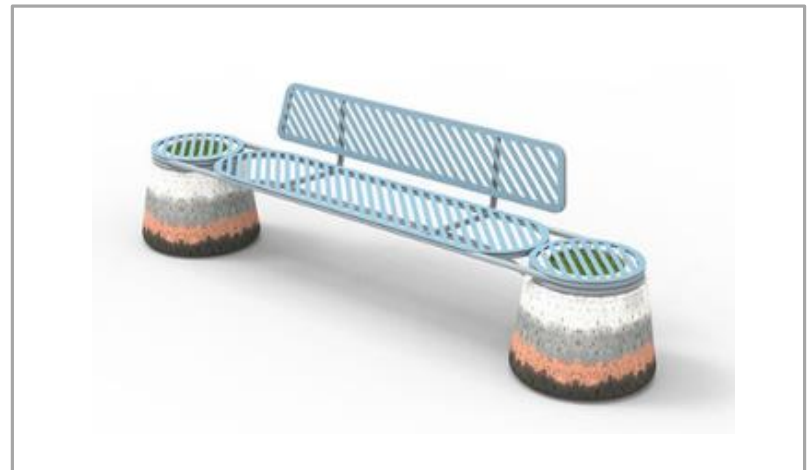
MUVA BANK DIMENSIONS | 2516x 522 x 709mm
