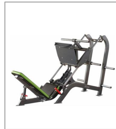
XLINE XR202 LEG PRESS EXERCISE MACHINE (45 degrees) DIMENSIONS | 2476x1212x1493 mm
