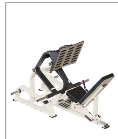
VERTI V202 ANGLE LEG PRESS EXERCISE MACHINE DIMENSIONS | 2353x1852x1574 mm
