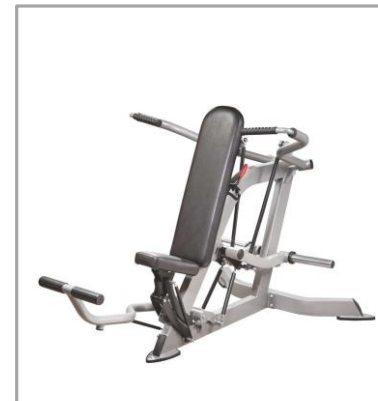
XLINE X205 OVERHEAD PRESS EXERCISE MACHINE DIMENSIONS | 1860x1155x1190 mm
