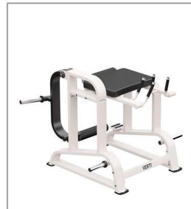
VERTI V224 REVERSE HYPEREXTENSION DIMENSIONS | 1140x1520x1270 mm
