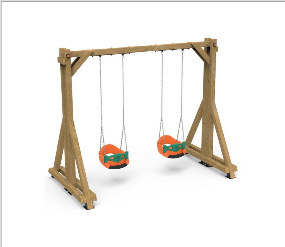
PK. 26001 DIMENSIONS | 1760 X 3100 X 2450 mm AGE GROUP | 3-15 yrs
