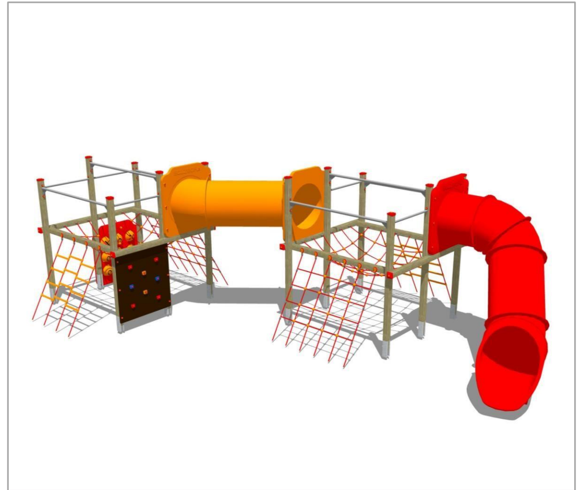
THREE TOWERS FUN OASIS XOA103L WITH BRIDGES AND TUBE SLIDE DIMENSIONS | length: 872 width: 824 age of use: > 3
